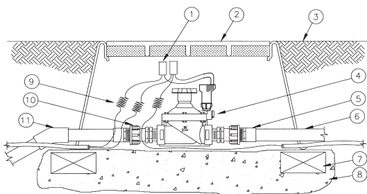
4 170S-150 1-1/2" and 170S-200 2" REMOTE CONTROL VALVE FOR LEIT CONTROLLER ASSEMBLY
