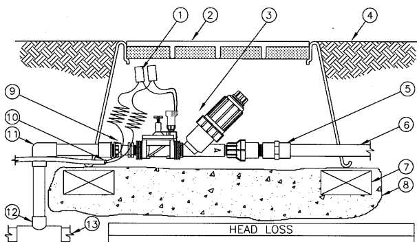
4 170S-150 1-1/2" and 170S-200 2" REMOTE CONTROL VALVE FOR LEIT CONTROLLER ASSEMBLY
